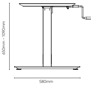
Winder Adjust (Speed 5 mm/Turn)
